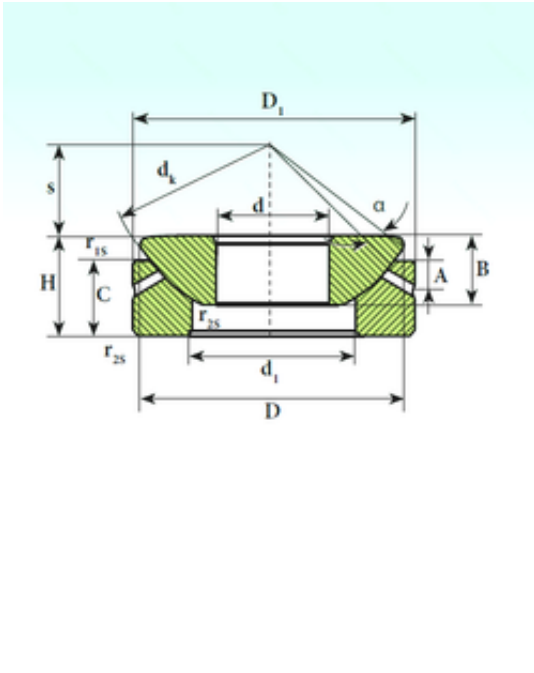
GX 70 S Bearing 2D drawings and 3D CAD models
